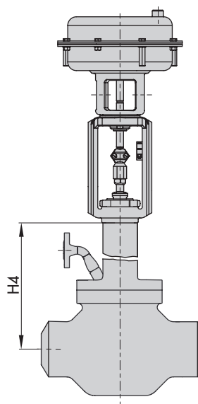
Type 3281-7 with insulating section and welding ends
