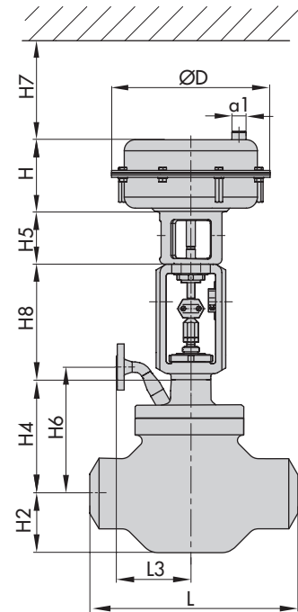
Type 3281-7 with welding ends
