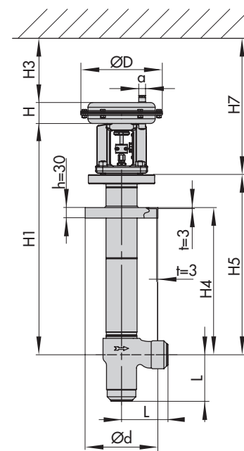
Fig. 7: Type 3248-1 Angle Valve
