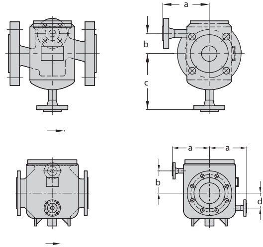
Type 3291 with heating jacket (dimensions on request)
