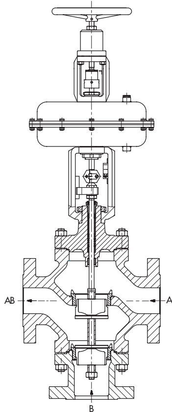
Fig. 2: Type 3253-1 Control Valve with Type 3271 Pneumatic Actuator and additional handwheel, body version for DN 50 to 500, plug arrangement for mixing service (anti-rotation fixture for DN 50 and larger)
