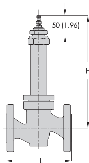
Fig. 3-2: Dimensional drawing
