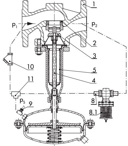
Type 2422 Valve, DN 65 to 100, balanced by a bellows, with Type 2420 Actuator
