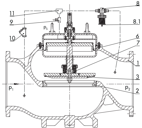
Type 2423 Valve, DN 125 to 400, balanced by a diaphragm
