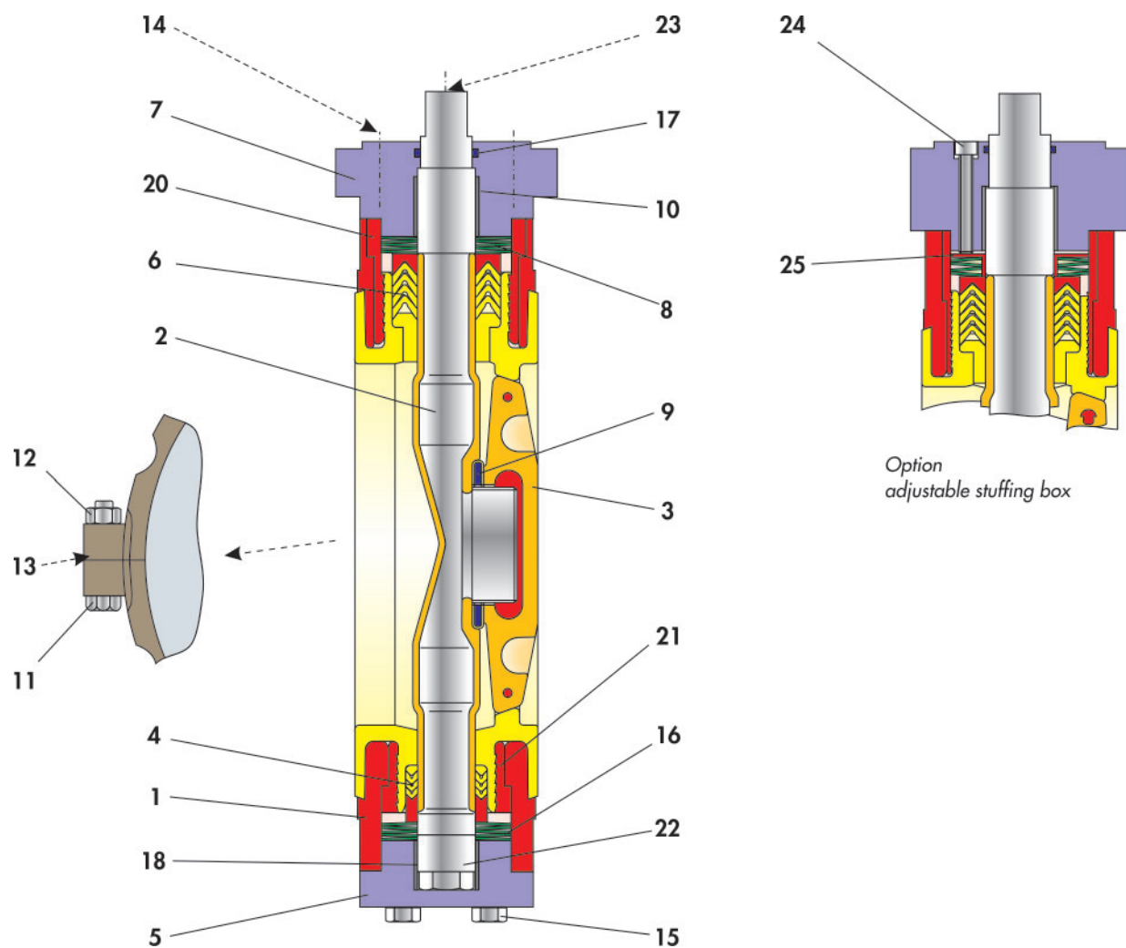
Fig. 3: M-PTFE-lined Butterfly valve
