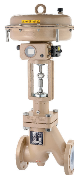
Bild 2: PFEIFFER Type 01b Control Valve, DN 80 with SAMSON actuator
